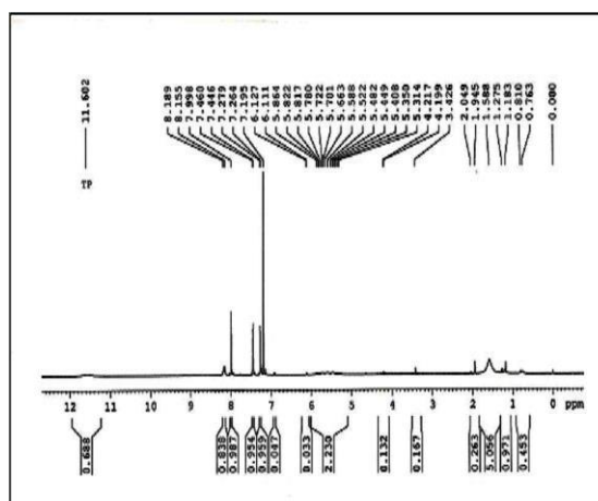
Fig 2: FTIR-Raman Spectroscopy of Thieno [2, 3-D] Pyrimidin-4-One
